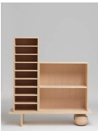
CABINET #3 ART. C.13.135.F1 Shelves: Wood Top: Wood, Foot: Wood W:1350 D:500 H:1416 mm
